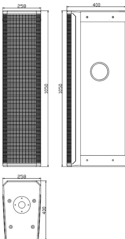
KAMIQ - K9SAT DIMENSIONS
